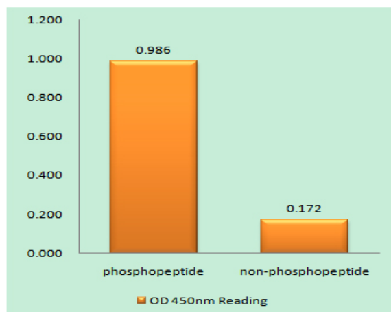
Enzyme-Linked Immunosorbent Assay (Phospho-ELISA) for Immunogen Phosphopeptide (Phospho-left) and Non-Phosphopeptide (Phospho-right), using VEGFR2 (Phospho-Tyr1214) Antibody
