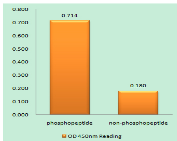
Enzyme-Linked Immunosorbent Assay (Phospho-ELISA) for Immunogen Phosphopeptide (Phospho-left) and Non-Phosphopeptide (Phospho-right), using CrkII (Phospho-Tyr221) Antibody
