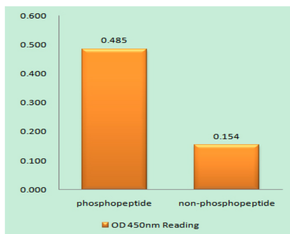
Enzyme-Linked Immunosorbent Assay (Phospho-ELISA) for Immunogen Phosphopeptide (Phospho-left) and Non-Phosphopeptide (Phospho-right), using Estrogen Receptor-alpha (Phospho-Tyr537) Antibody
