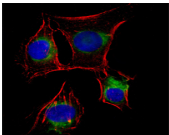
Immunofluorescence analysis of EC cells using NGFR p75 Monoclonal Antibody (green). Red: Actin filaments have been labeled with DY-554 phalloidin. Blue: DRAQ5 fluorescent DNA dye.
