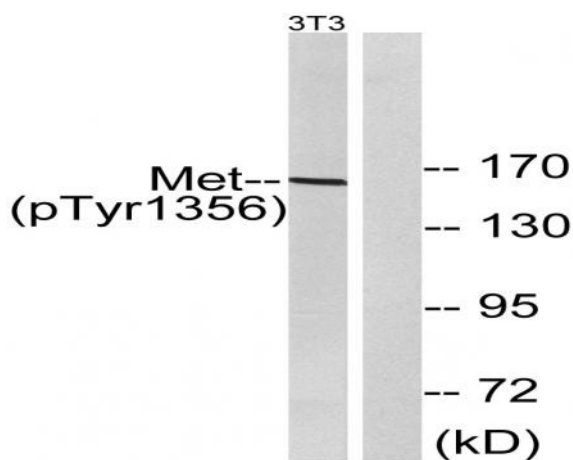
Western blot analysis of lysates from NIH/3T3 cells, using Met (Phospho-Tyr1356) Antibody. The lane on the right is blocked with the phospho peptide.
