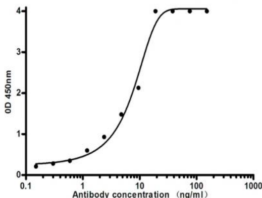
Indirect ELISA assay for Mouse Anti-human IgM mouse mAb. Antigen coating concentration: 2ug/ml.
